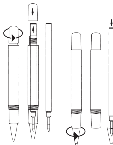
Tintenroller
